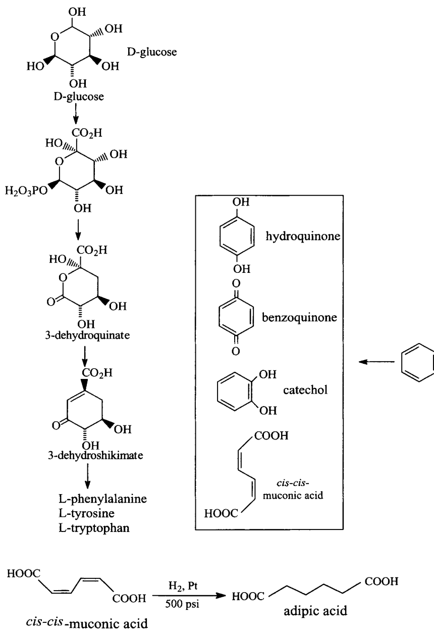
FIGURE 12.7. Draths–Frost synthesis of adipic acid (compare to the benzene-based synthesis).
