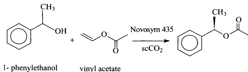
FIGURE 12.20. Esterification reaction using an enzyme and \text{scCO}_2 . (Source: Overmeyer, 1999).
