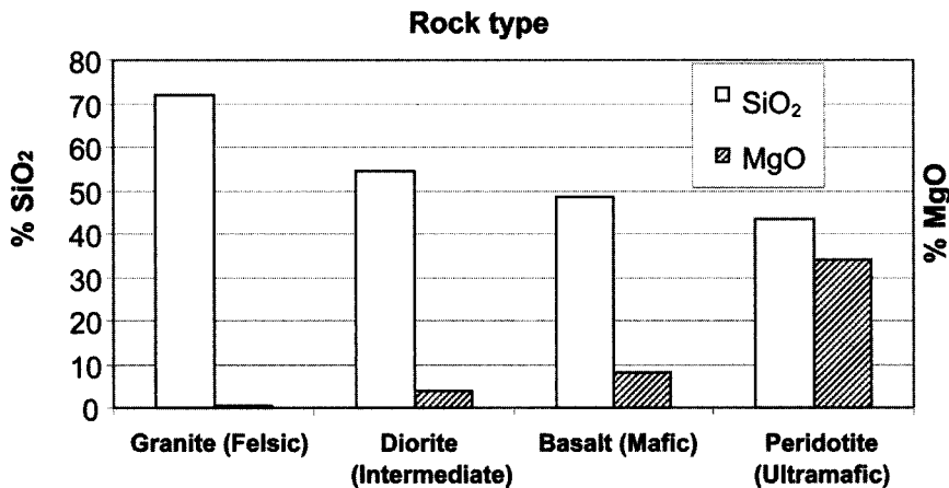
FIGURE 5.1. Relationship between the SiO 2 and MgO contents of igneous rocks.
