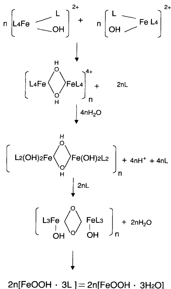
FIGURE 5.7. Simplified precipitation scheme of \text{Fe}^{3+} + \text{OH}^- . Here, L denotes \text{H}_2\text{O} .
