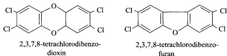
FIGURE 9.15. Examples of TCCD and TCBF.
