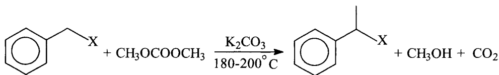
FIGURE 12.4. Dimethyl carbonate as an alkylating agent.
