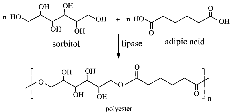
FIGURE 12.9. An enzymatic polymerization reaction (water is also a product).
