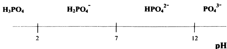
FIGURE 8.5. Predominance-zone diagram for phosphates.
