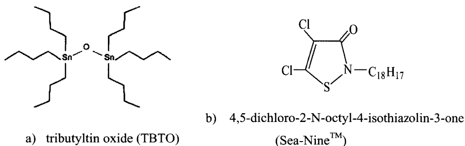
FIGURE 12.1. Antifouling agents.
