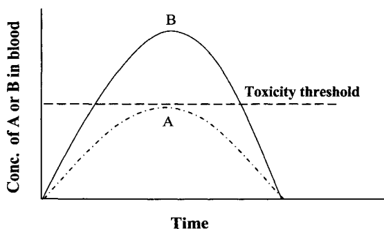
FIGURE 9.24. Effect of different doses over time for toxicants A and B. (Adapted from Kamrin, 1988).
