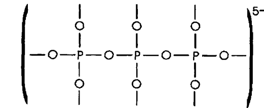
FIGURE 8.4. Chemical structure of a polyphosphate anion.
