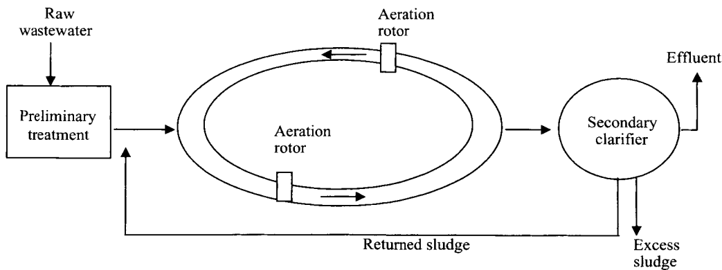
FIGURE 11.3. Oxidation ditch.
