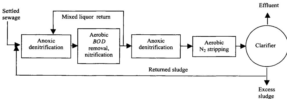
FIGURE 11.13. The Bardenpho process.
