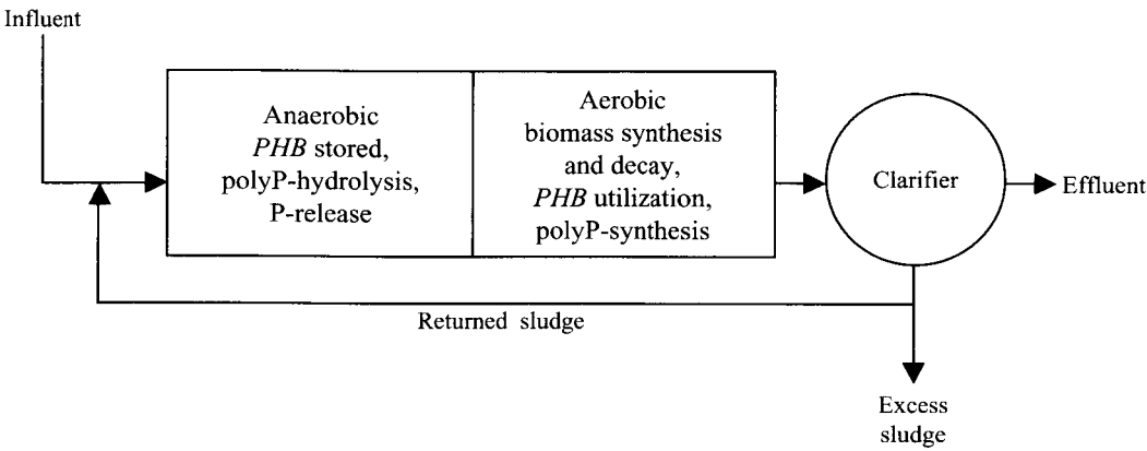
FIGURE 11.14. A/O process for phosphorous removal.
