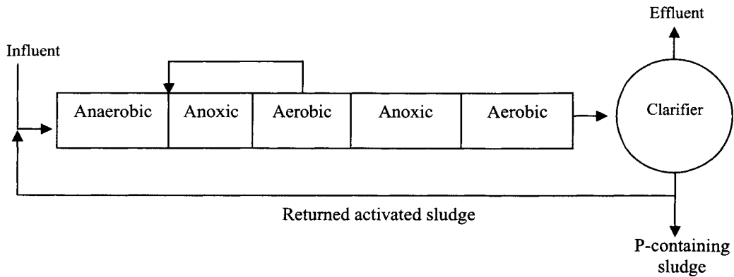
FIGURE 11.16. Modified Bardenpho process for phosphorous and nitrogen removal.
