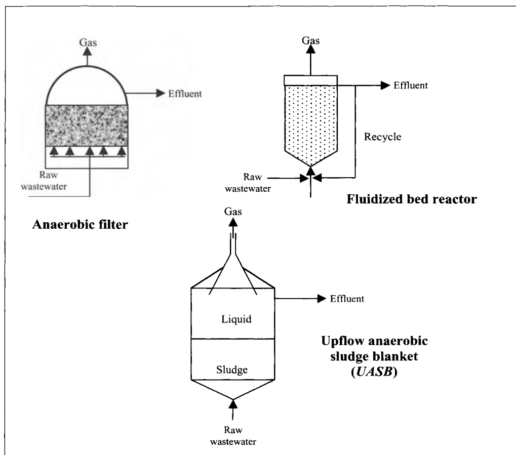
FIGURE 11.8. Anaerobic processes.
