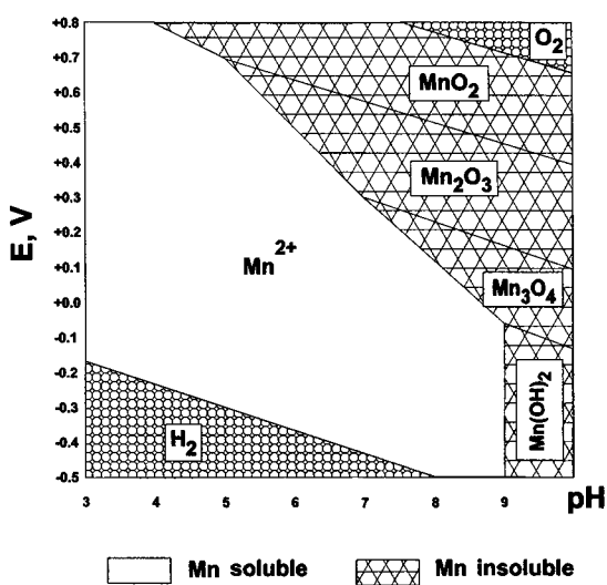
FIGURE 6.8. E -pH diagram for Mn.
