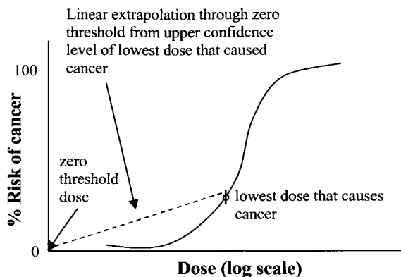
FIGURE 9.34. Extrapolation in the LMS model.
